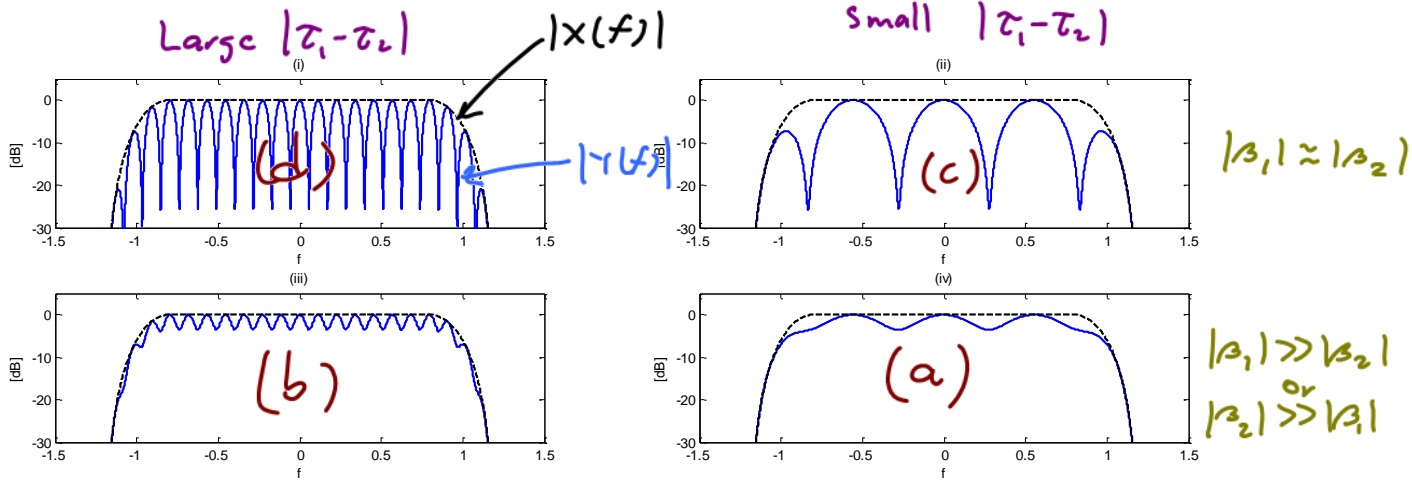
Figure 16: Frequency selectivity in the receive spectra (blue line) for two-path channels.
