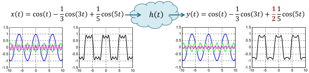
Figure 10: Channel with high-frequency attenuation
