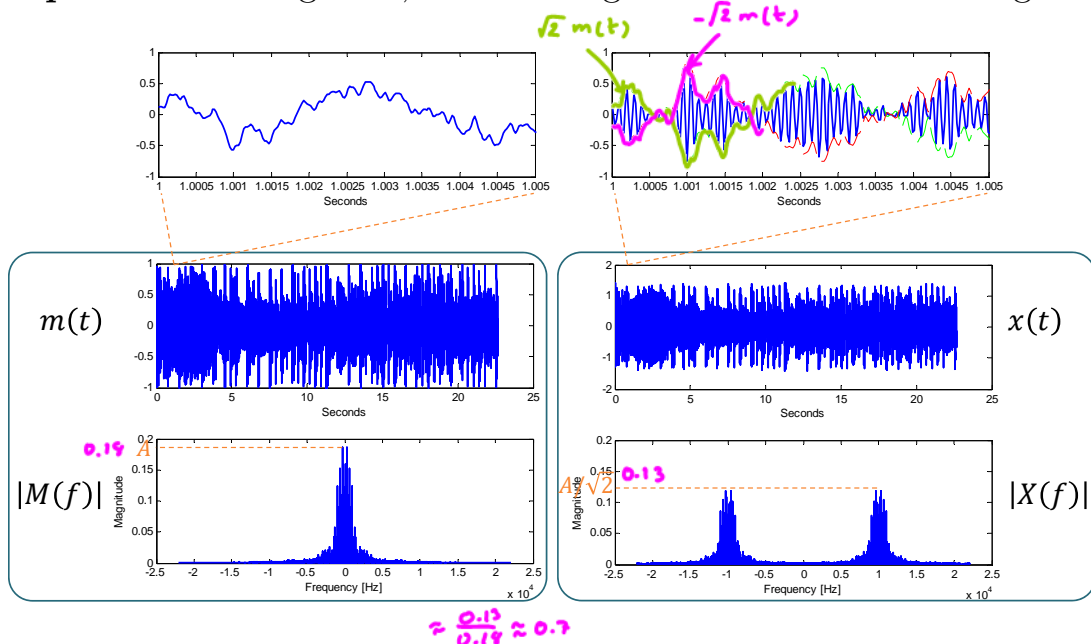
Figure 7: Signals in a simple modulator when an audio signal is used as its message.
