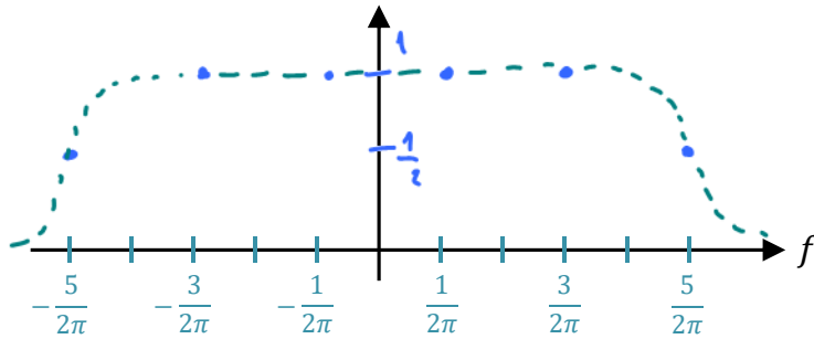
Figure 11: An example of H(f) that satisfies the input-output relationship in Figure 10.
