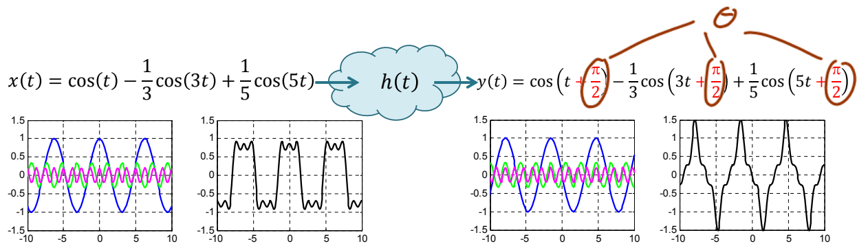
Figure 12: Channel with constant phase shift
