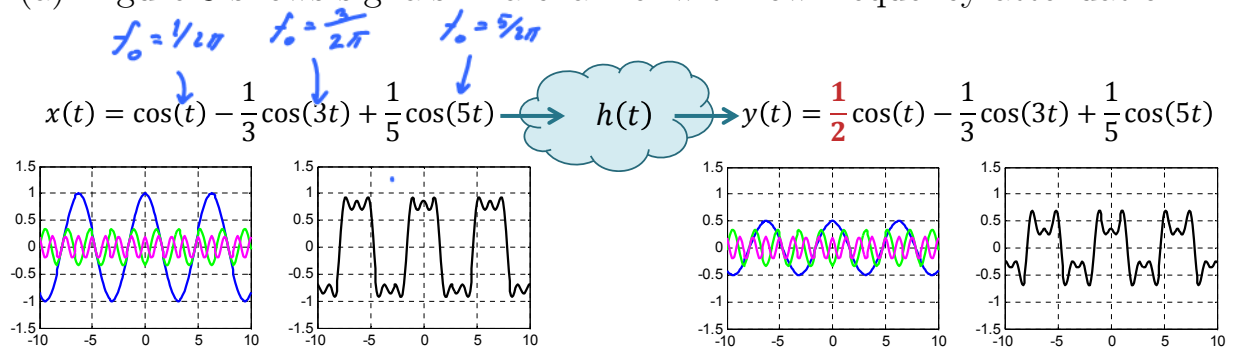
Figure 8: Channel with low-frequency attenuation
