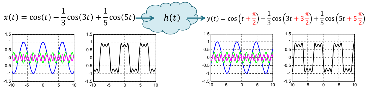
Figure 14: Channel with linear phase shift
